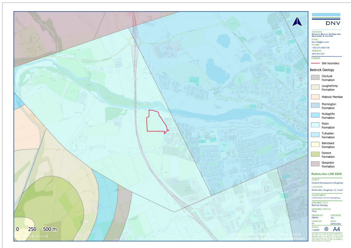
Figure 6-6. Bedrock Geology
