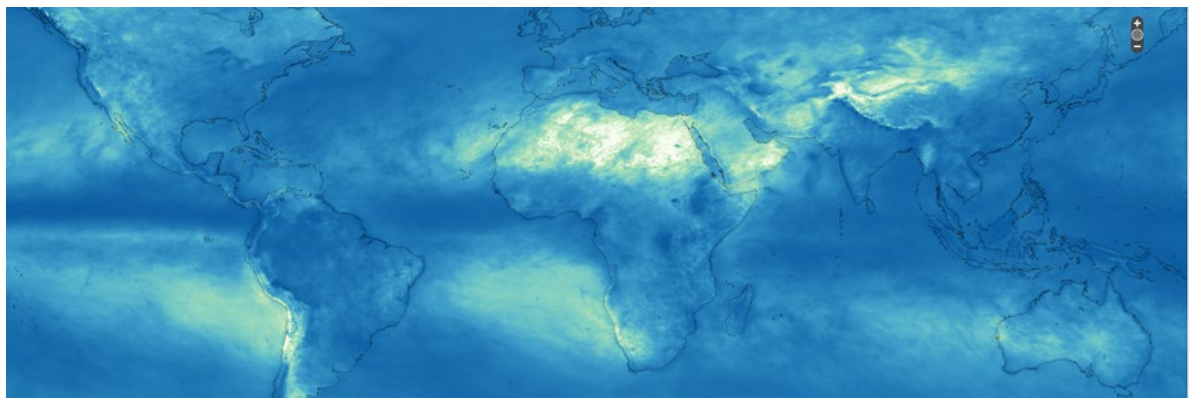
Figure 9.3 Multi-model ensembled rainfall projection for 2050 (SSP5-8.5)
