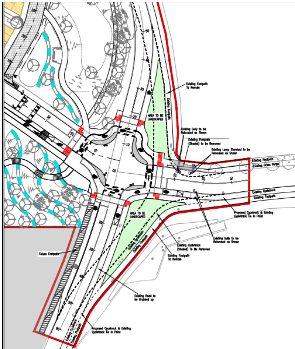
Figure 13-15 Proposed Junction 1 (Rathmullan Road / Local Road/Site access road) upgrade)
