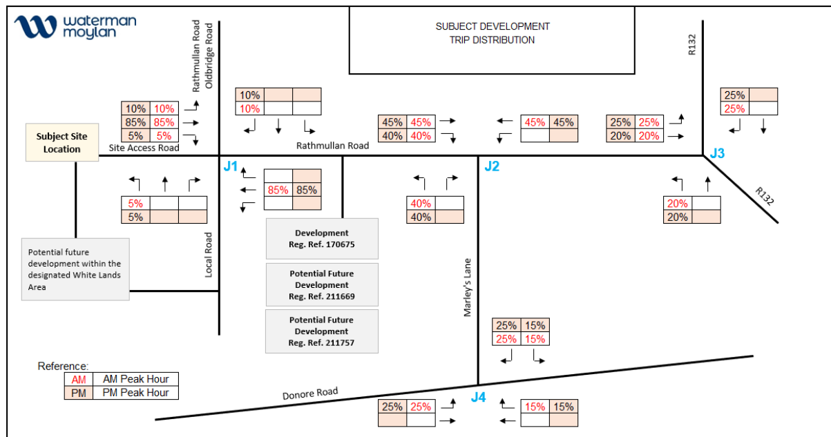
Figure 13-21 Subject Site Trip Distribution
