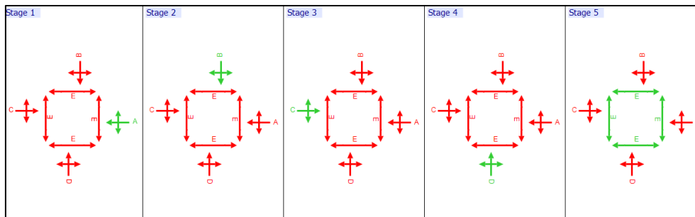
Figure 13-33 Junction 1 – Stage Sequence
