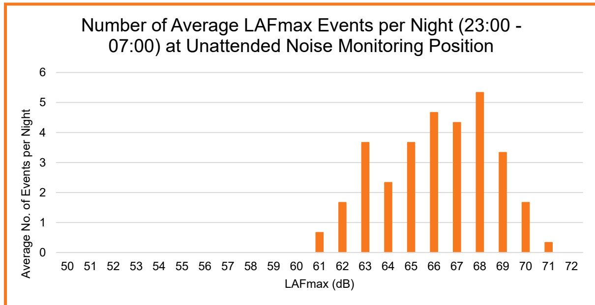
Figure 10-5 Average recorded L_{AFmax} events per night based on 15min measurement intervals
