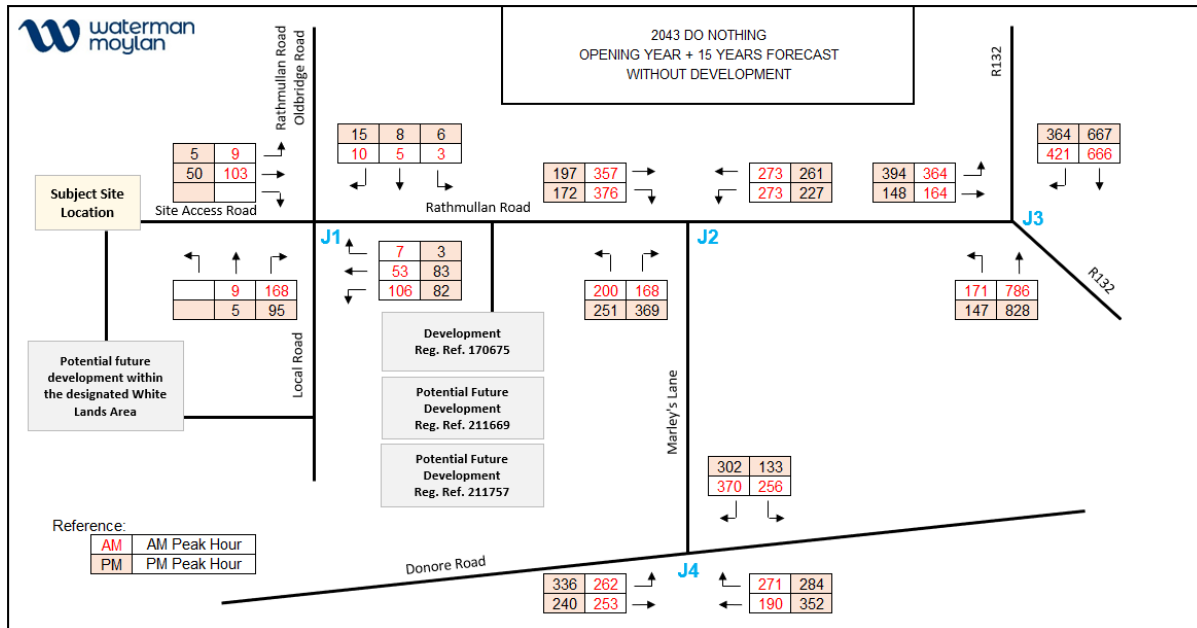
Figure 13-29 Traffic Flows - 2043 DO NOTHING - Opening year + 15 years, Without Development
