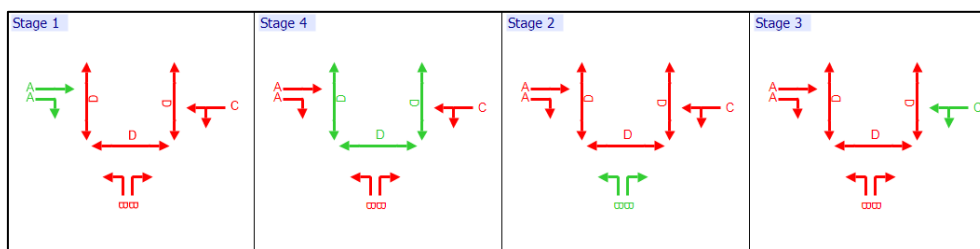
Figure 13-34 Junction 2 – Stage Sequence
