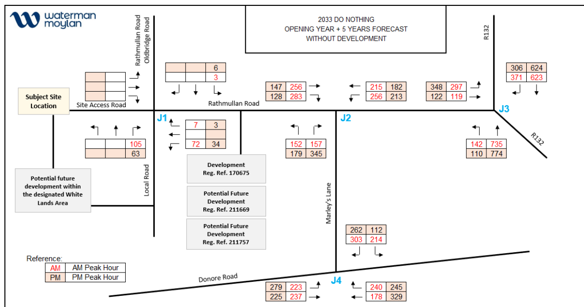
Figure 13-28 Traffic Flows - 2033 DO NOTHING - Opening year + 5 years, Without Development
