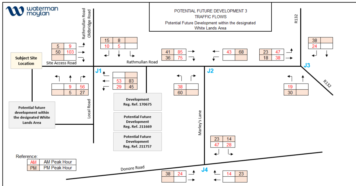
Figure 13-25 Potential Future Developments - Traffic Flows – Potential Future Development within the designated White Lands Area
