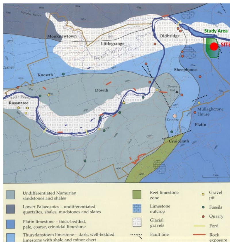
Figure 12-2 Underlying Geology in Area of the Proposed Development Site (Stout, 2002)
