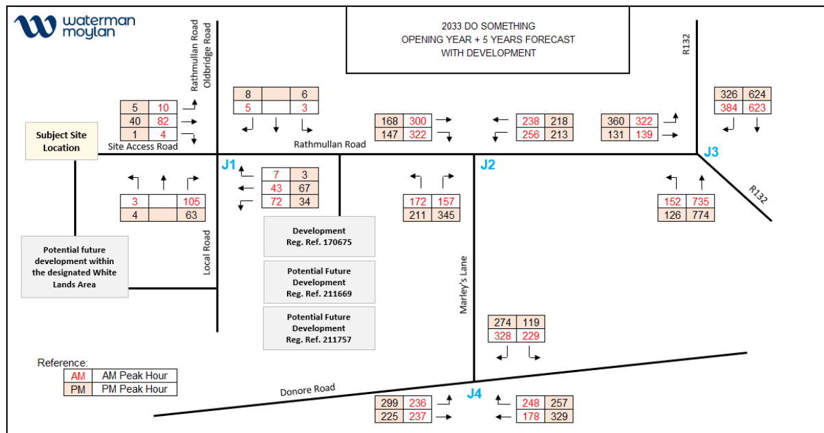
Figure 13-31 Traffic Flows - 2033 DO SOMETHING - Opening year + 5 years, With Development
