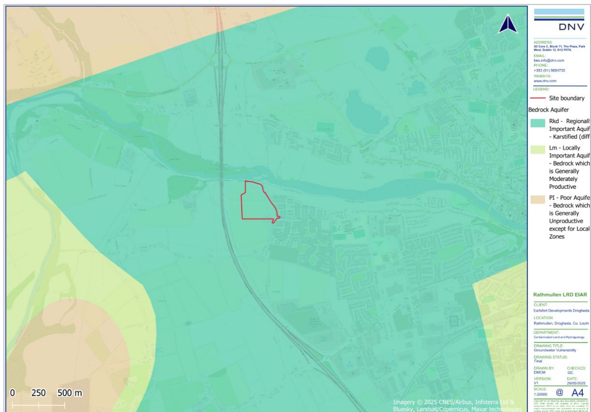
Figure 7-4. Aquifer Classification
