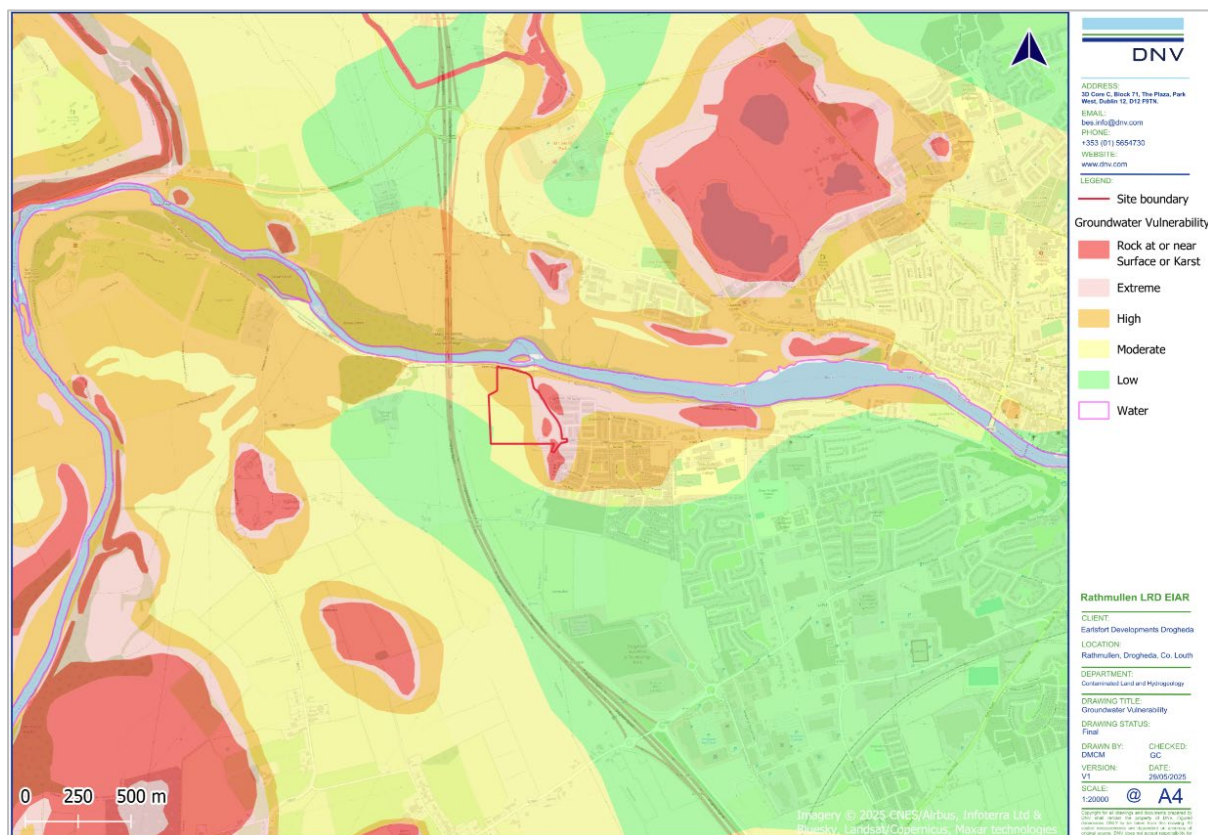
Figure 7-5. Groundwater Vulnerability
