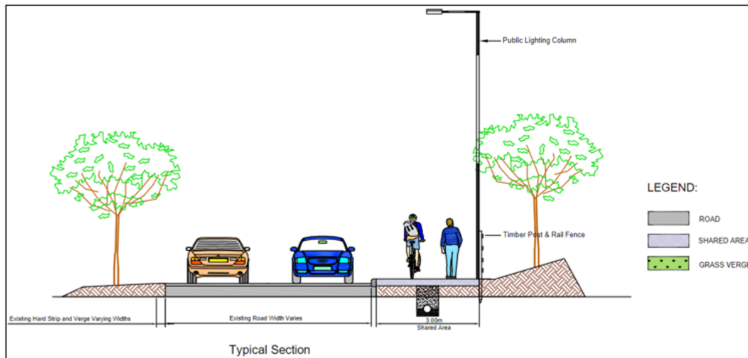
Figure 13-13 Rathmullan Road – Proposed Shared Footway / Cycleway – Typical Section (Source: Construction of a Shared Cycleway/Footway on the Rathmullan Road)
