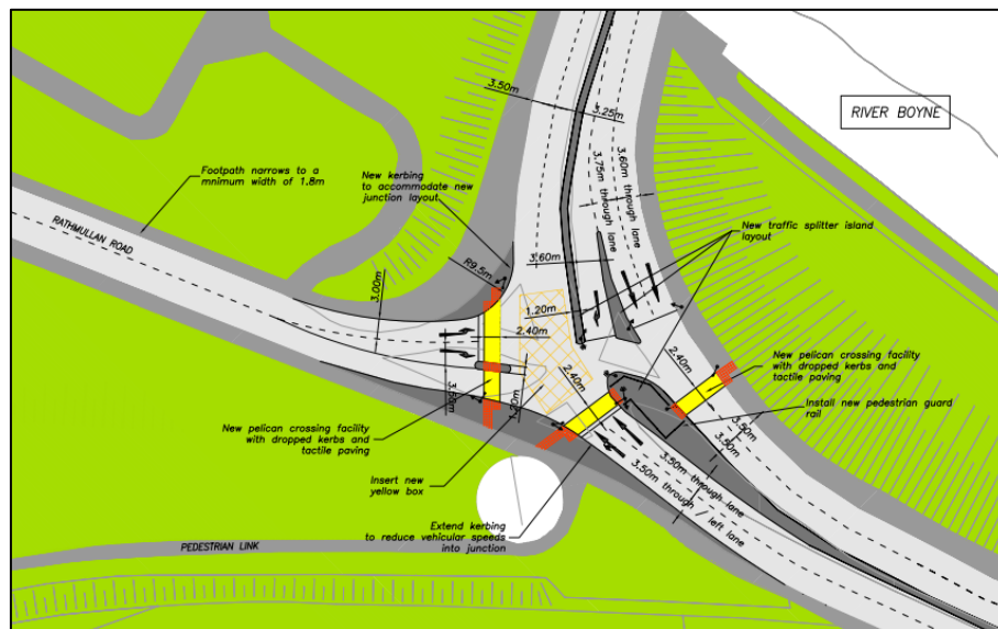
Figure 13-16 Proposed Junction 3 (Rathmullan Road / R132) Upgrade (Source: Transportation Study (December 2006))
