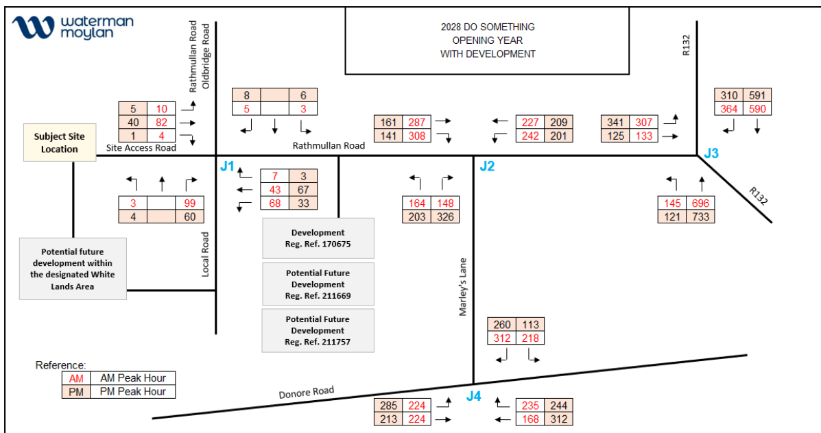
Figure 13-30 Traffic Flows - 2028 DO SOMETHING - Opening year, With Development
