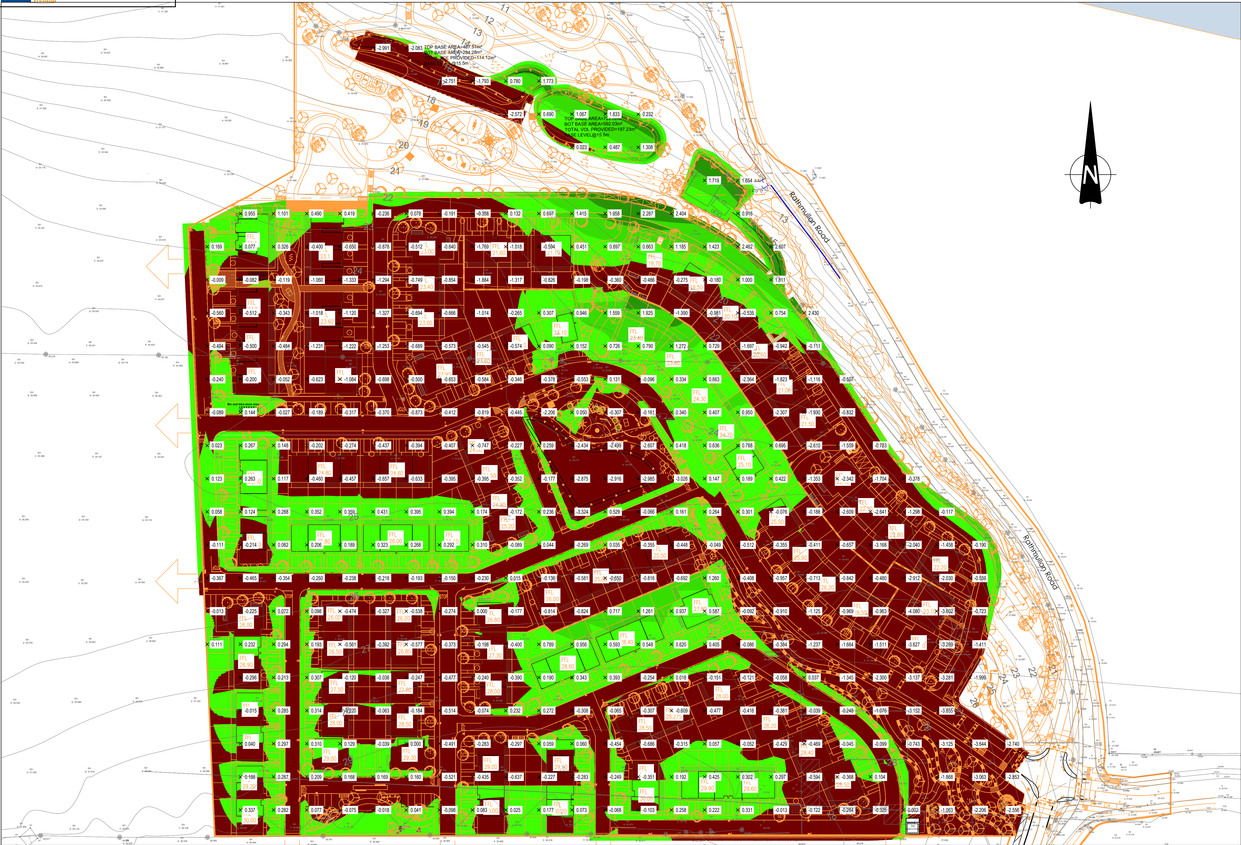
PLAN VIEW – CUT AND FILL ANALYSIS
