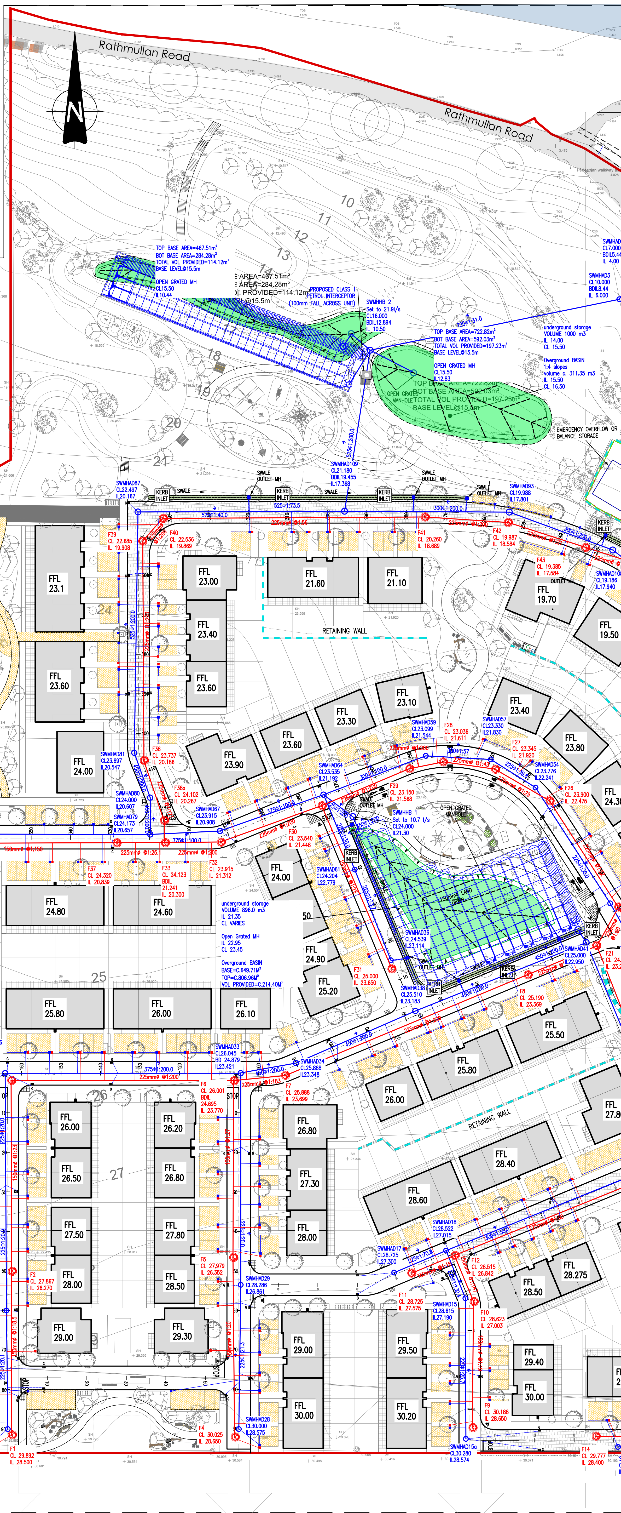
PROPOSED DRAINAGE LAYOUT - SHEET 2 OF 2
