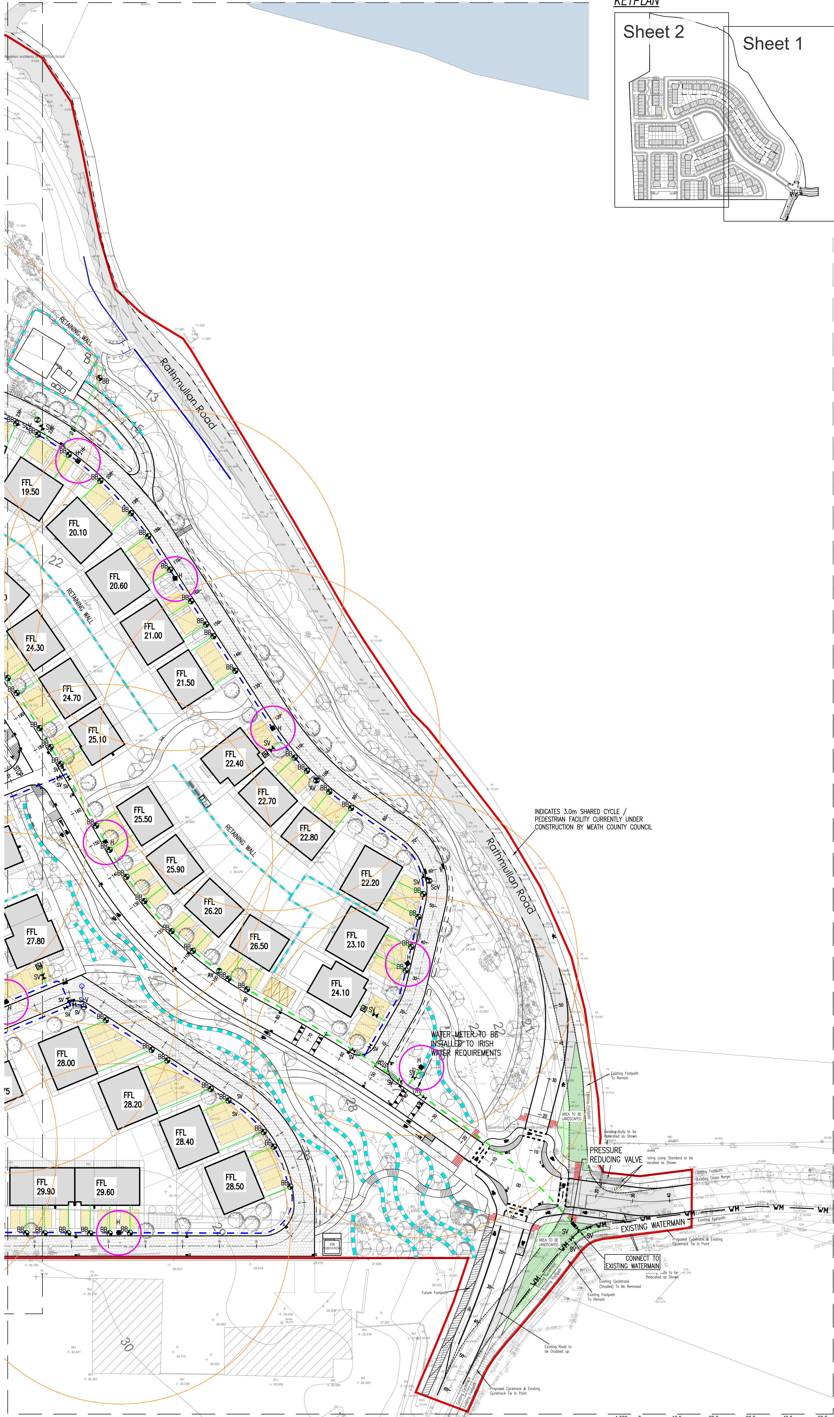
PROPOSED WATER SUPPLY LAYOUT – SHEET 1 OF 2
